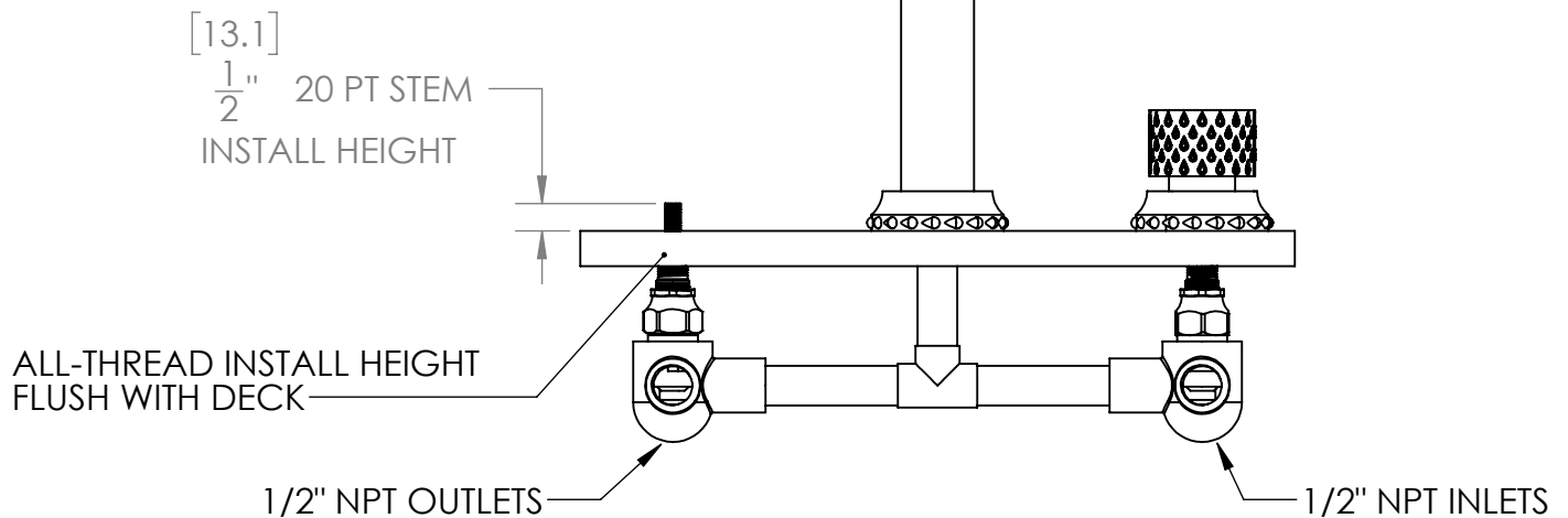
SOFT TOUCH DRAIN ASSEMBLY P/N 18.11.052
